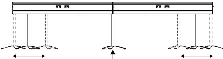
Multiple Service Spine leg placement
